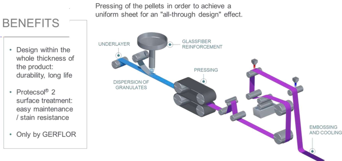
Figure 4: Pressing process' diagram
