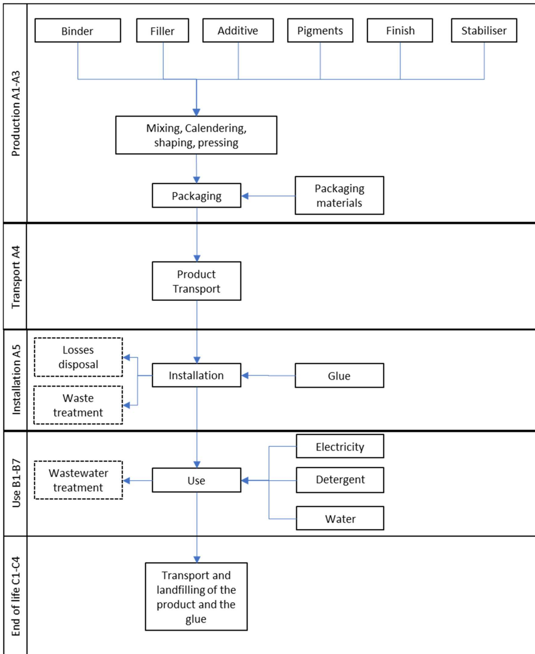
Figure 2 : Flow product diagram
